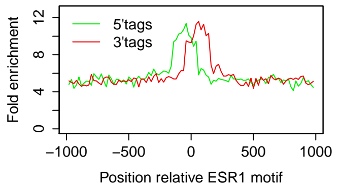
Xenograft_MCF7|ESR1|Vehicle|rep2
