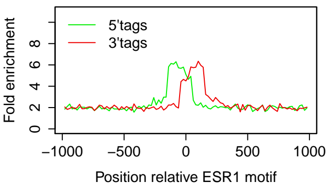
T47D|ESR1|Vehicle 3hr|rep1
