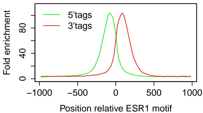
T47D|ESR1|Progesterone 3hr|rep2
