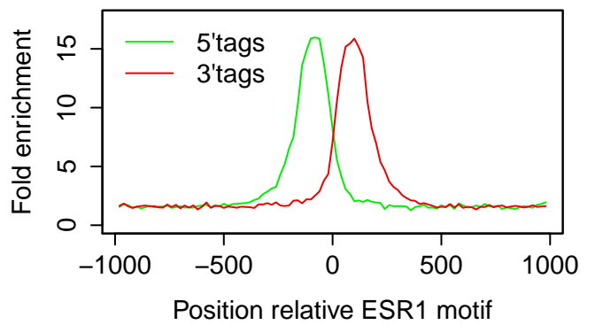
T47D|ESR1|E2+PG 3hr|rep2
