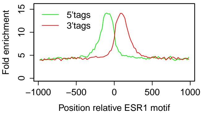
MCF7|ESR1|Vehicle 3hr|rep3
