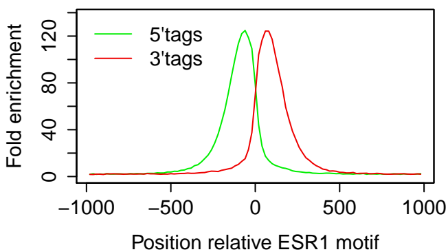
Xenograft_MCF7|ESR1|E2|rep13
