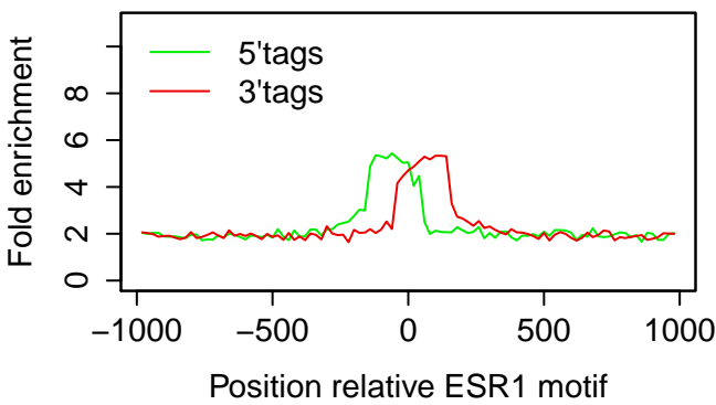
T47D|ESR1|Vehicle 3hr|rep2
