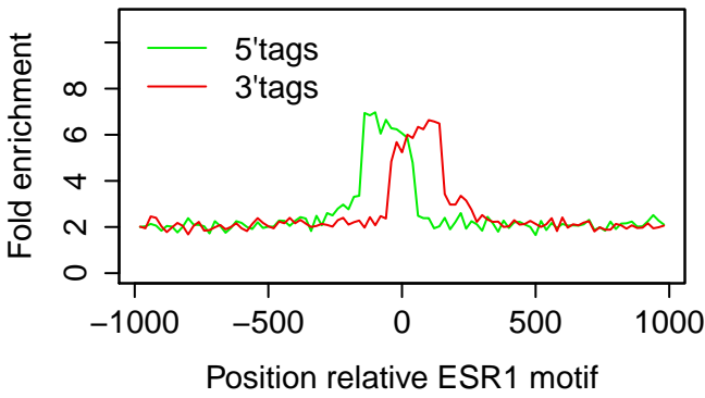
T47D|ESR1|PG 3hr|rep1
