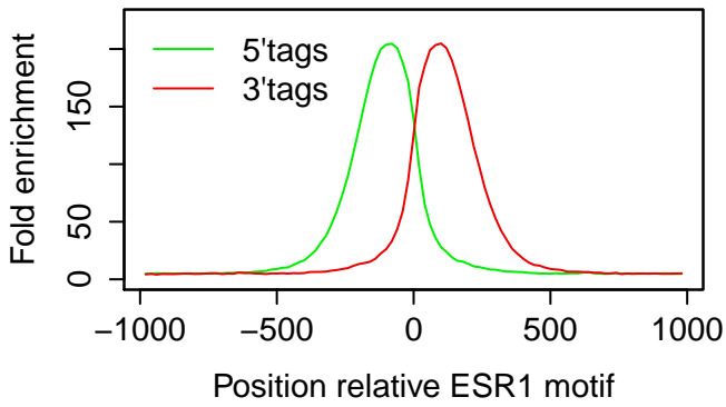
MCF7|ESR1|R5020 3hr|rep2
