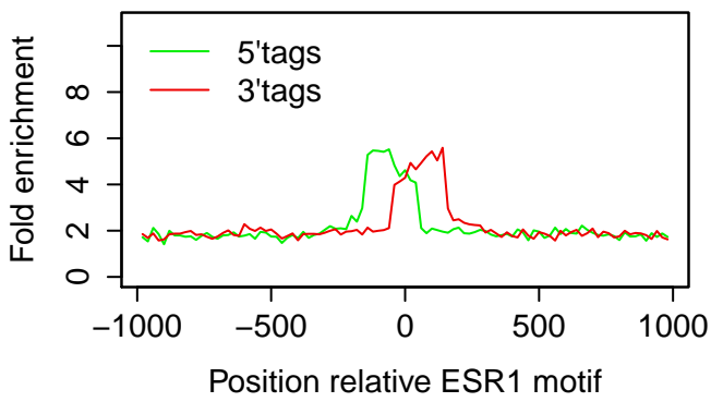
T47D|ESR1|PG 3hr|rep3
