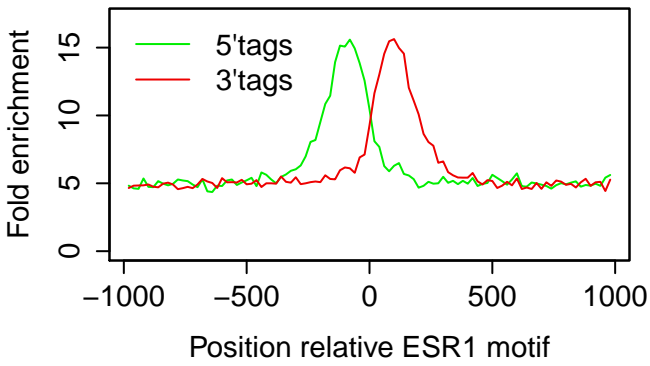
MCF7|ESR1|PG 3hr|rep2
