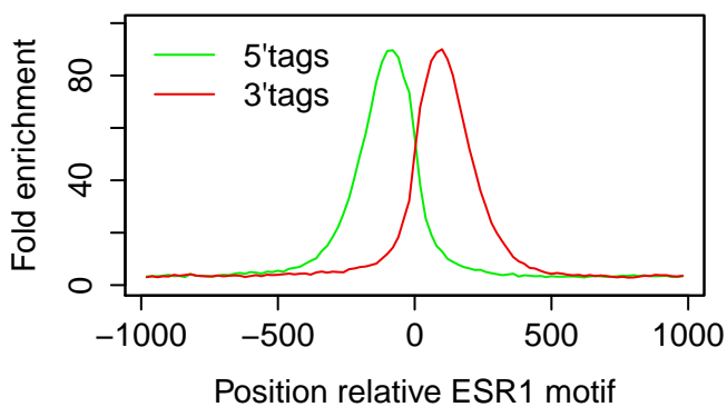
T47D|ESR1|R5020 3hr|rep1
