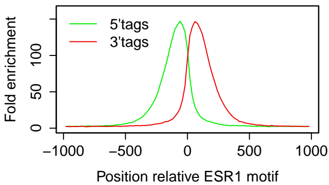
Xenograft_MCF7|ESR1|E2|rep11
