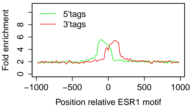
T47D|ESR1|PG 3hr|rep2
