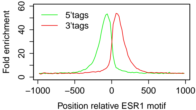
Xenograft_MCF7|ESR1|E2+PG|rep5
