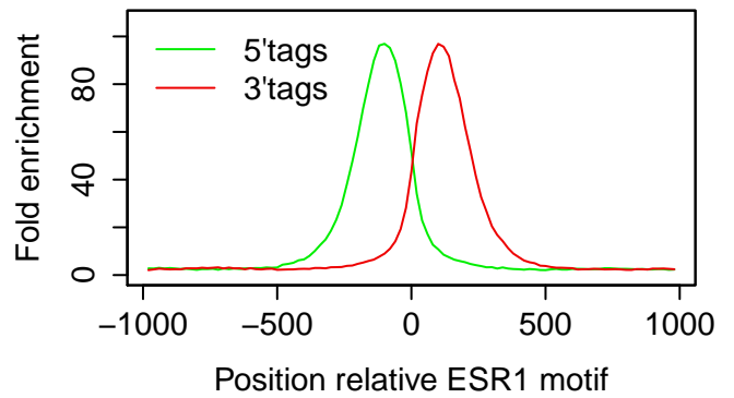
MCF7|ESR1|E2 3hr|rep1
