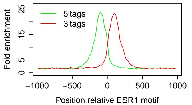
T47D|ESR1|E2 3hr|rep2
