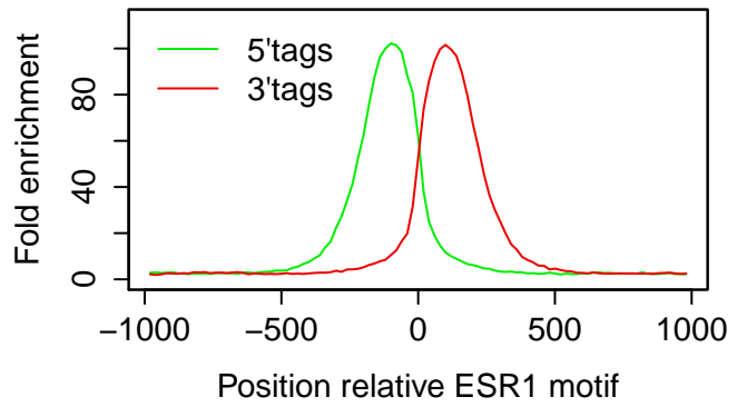
MCF7|ESR1|E2+PG 3hr|rep2
