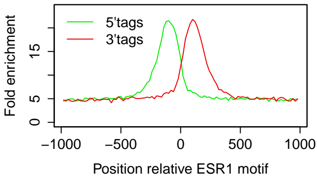
MCF7|ESR1|Vehicle 3hr|rep1
