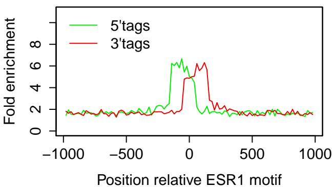
T47D|ESR1|Vehicle 3hr|rep3
