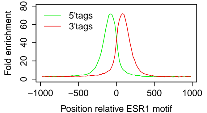
T47D|ESR1|R5020 3hr|rep2
