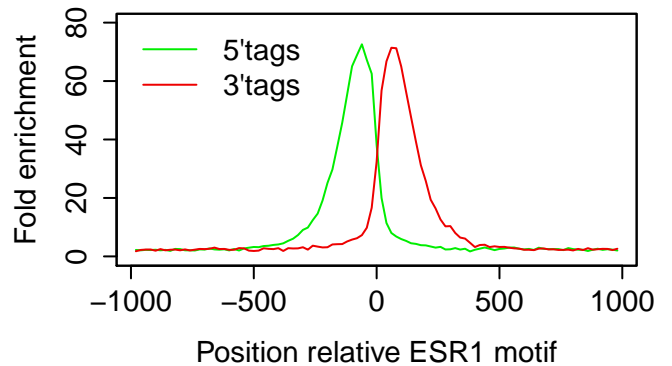
Xenograft_MCF7|ESR1|E2+PG|rep6
