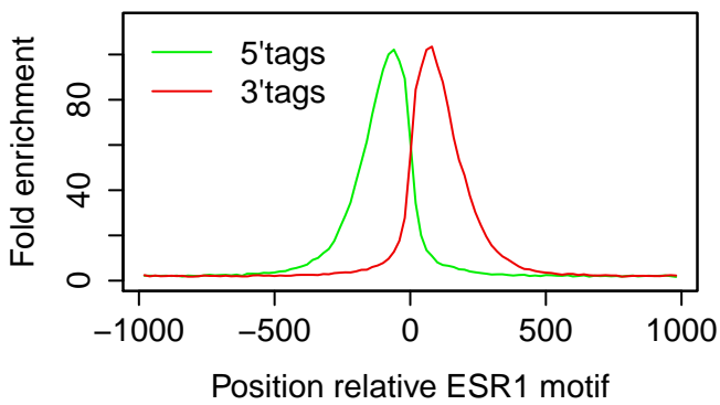
Xenograft_MCF7|ESR1|E2+PG|rep3
