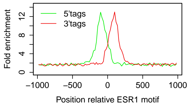
T47D|ESR1|E2+PG 3hr|rep3
