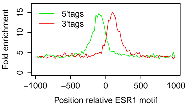
MCF7|ESR1|PG 3hr|rep3
