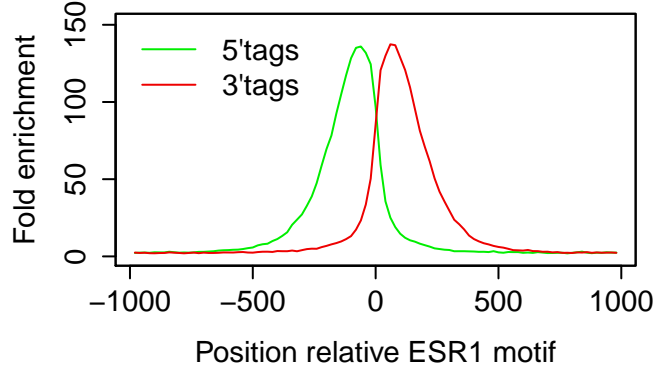
Xenograft_MCF7|ESR1|E2|rep14
