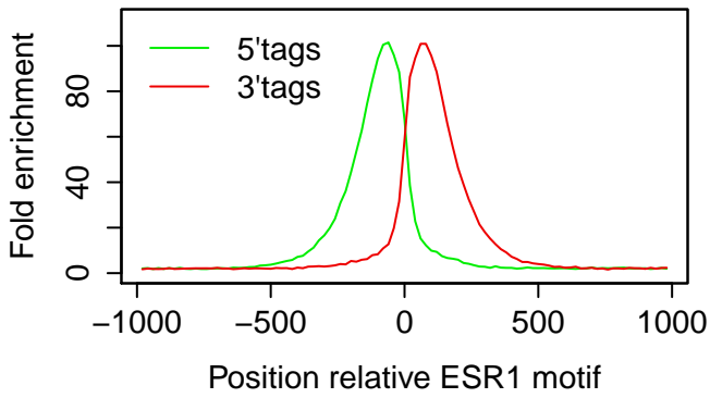
Xenograft_MCF7|ESR1|E2+PG|rep7
