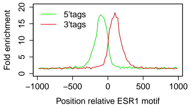
T47D|ESR1|E2 3hr|rep3
