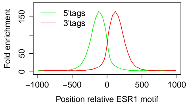
MCF7|ESR1|E2+PG 3hr|rep1
