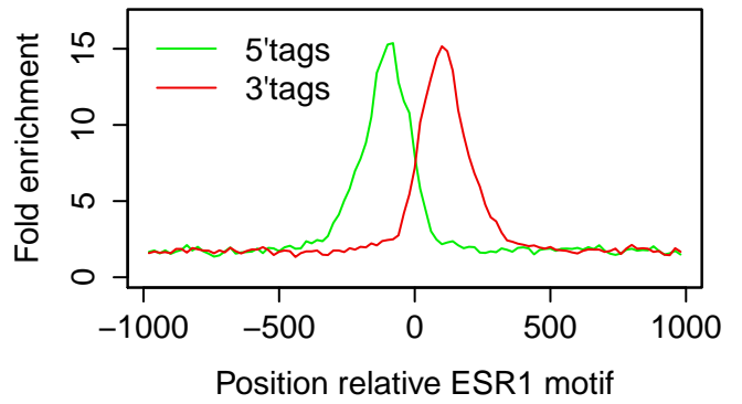
T47D|ESR1|E2+PG 3hr|rep1
