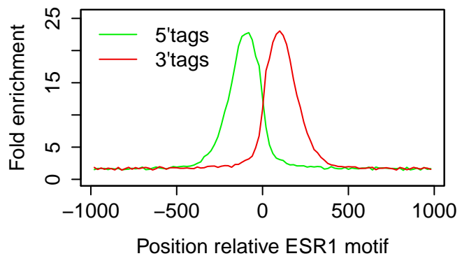
T47D|ESR1|E2 3hr|rep1
