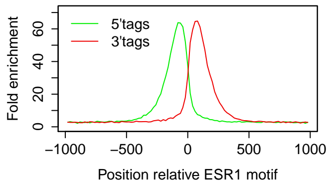
Xenograft_MCF7|ESR1|E2+PG|rep4
