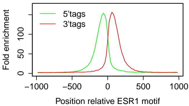
Xenograft_MCF7|ESR1|E2|rep9
