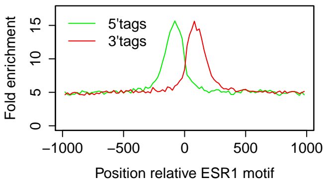
MCF7|ESR1|Vehicle 3hr|rep2
