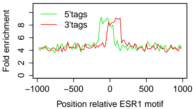
Xenograft_MCF7|ESR1|Vehicle|rep1
