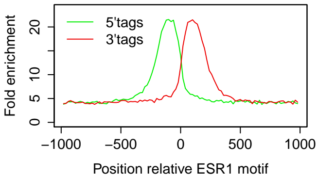
MCF7|ESR1|PG 3hr|rep1
