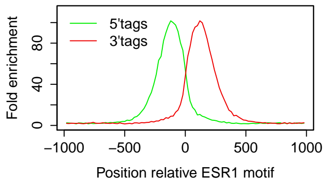
MCF7|ESR1|E2+PG 3hr|rep3
