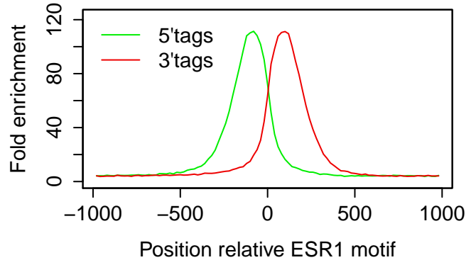
T47D|ESR1|Progesterone 3hr|rep1
