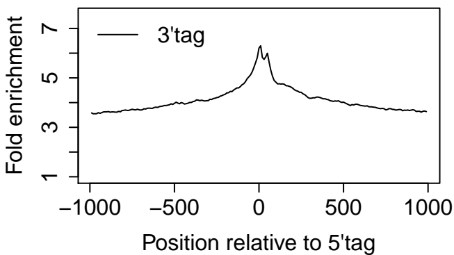
MCF7 | Input | |
