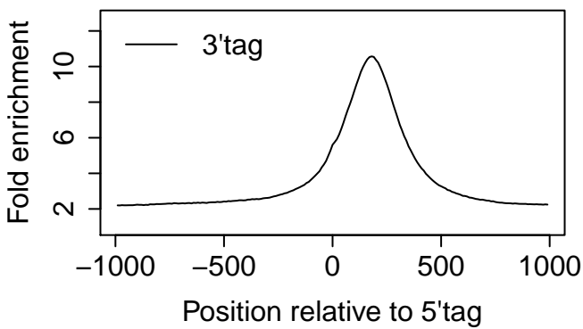
MCF7 | NR3C1 | |
